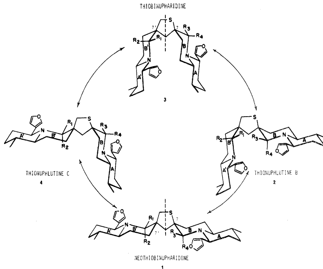
Figure 1. The four stereochemical classes of Nuphar thiaspirane alkaloids showing conceptual interconversion achieved through rotating AB and A'B' quinolizidine ring systems about C-7 and 8-7', respectively. Dashed vertical lines represent "pseudo- C_2 " axes which distinguish the "pseudosymmetrical" types.
